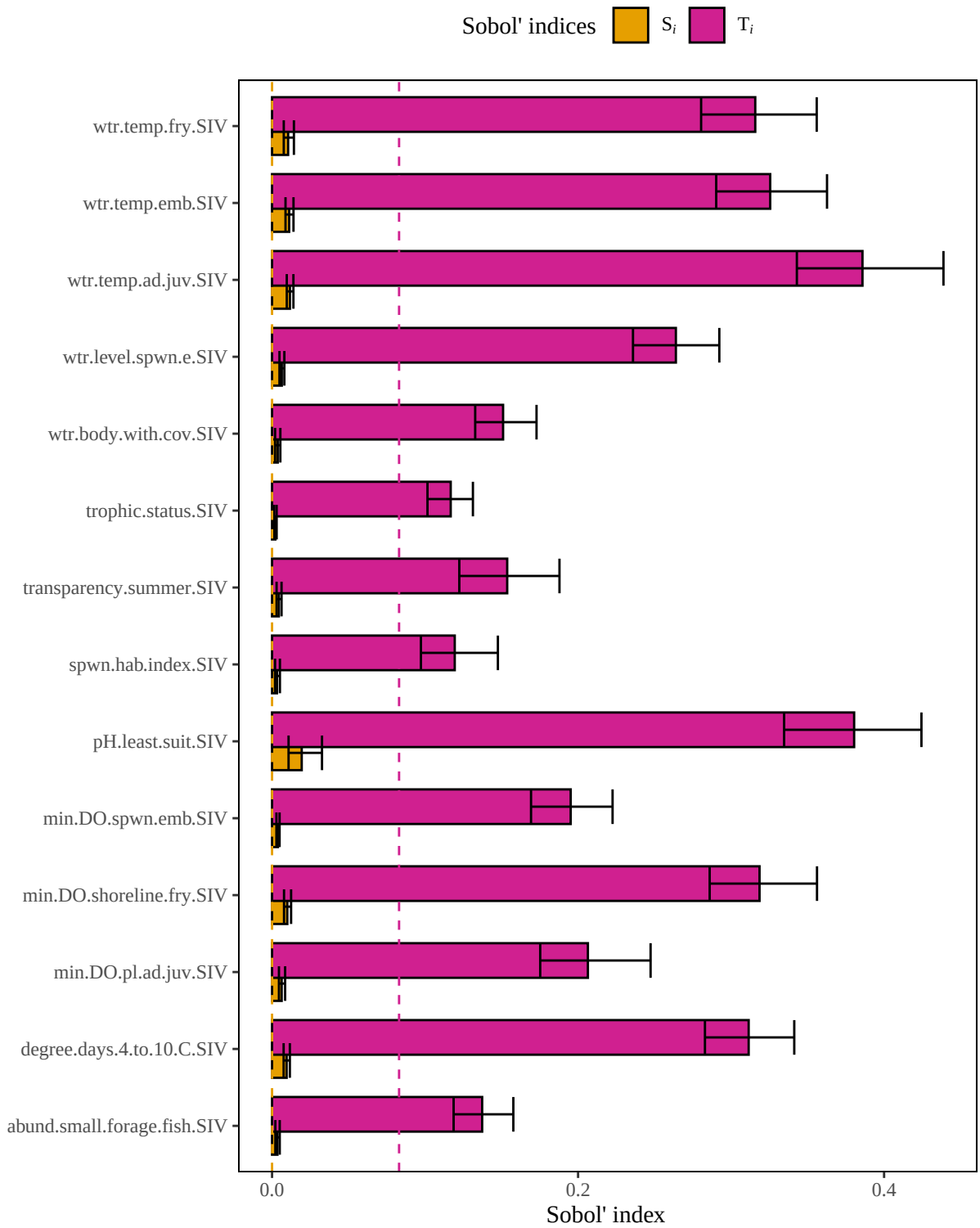
Figure 7. Results of a sensitivity analysis for the walleyeLacSecchiLtoe3.4m model based on a multiplicative mean structure. Dashed lines represent baseline numerical approximation error for S_i and T_i ( i.e. , dummy variables).
