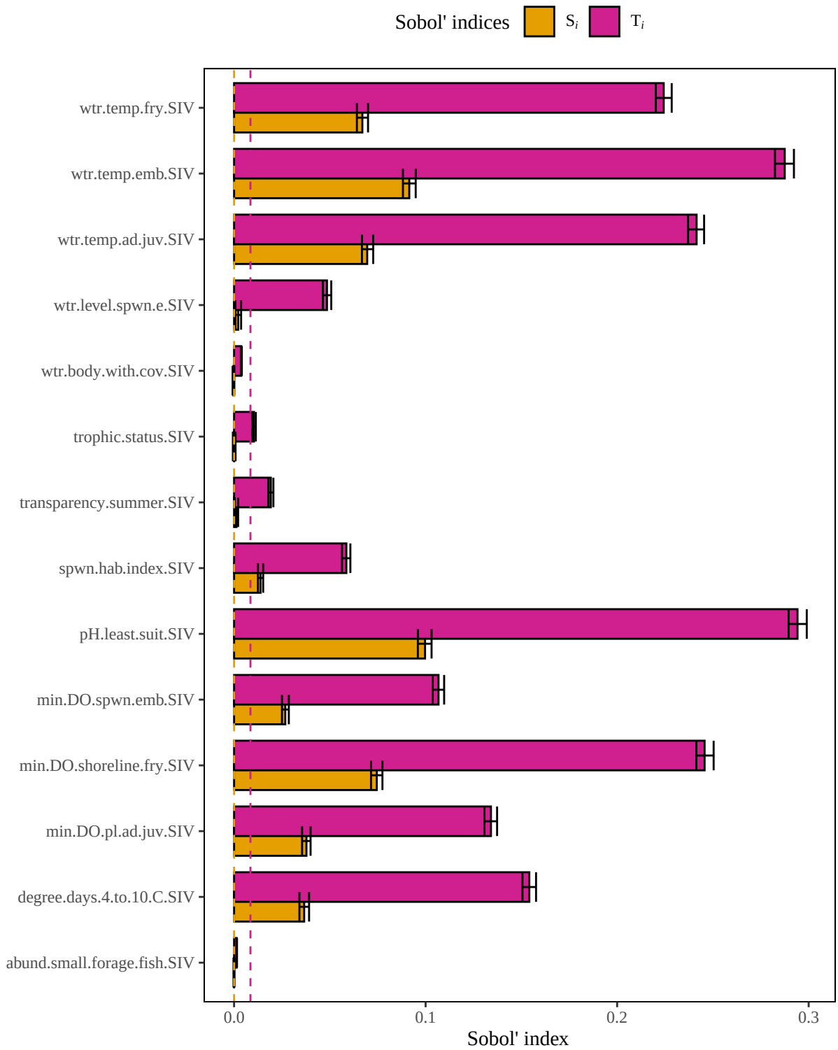
Figure 3. Results of a sensitivity analysis for the walleyeLacSecchiLtoe3.4m model based on the original author-specified model outlined in McMahon et al. (1984). Dashed lines represent baseline numerical approximation error for S_i and T_i ( i.e. , dummy variables).
